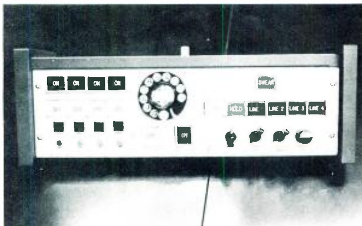
Fig. 2 Main switcher of the full-service system.
