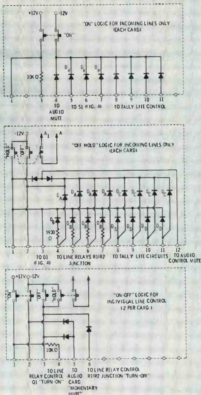
Fig. 6 Diode logic is laid out on 12-pin vector cards. Circled numbers are terminals. Diodes are shown for four incoming lines, and lettered to refer to Fig. 4.
